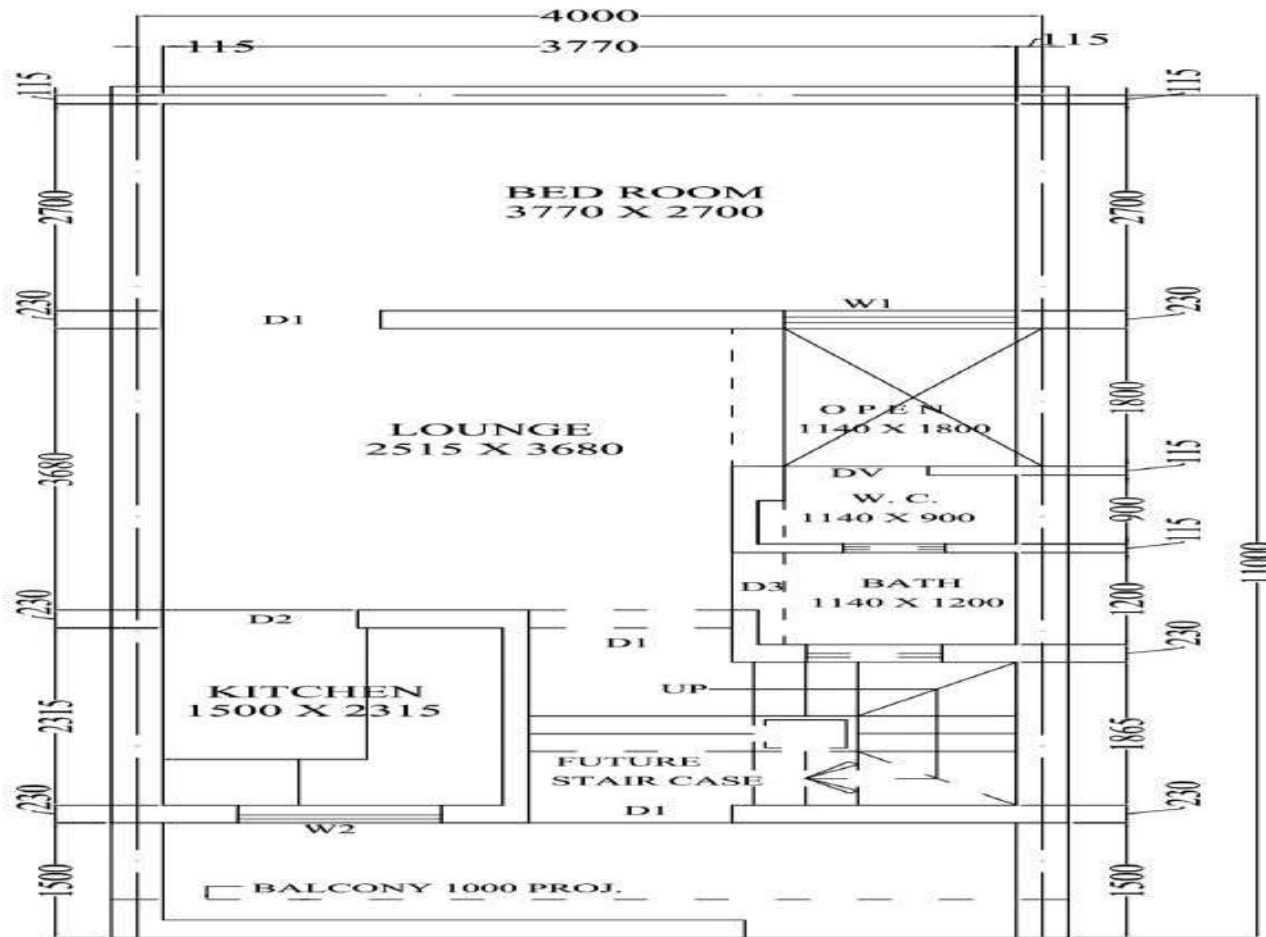
GROUND FLOOR PLAN 4.0 X 11.0 M (E.W.S.)
