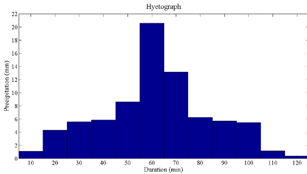
Figure C.2 Rainfall Hyetograph
