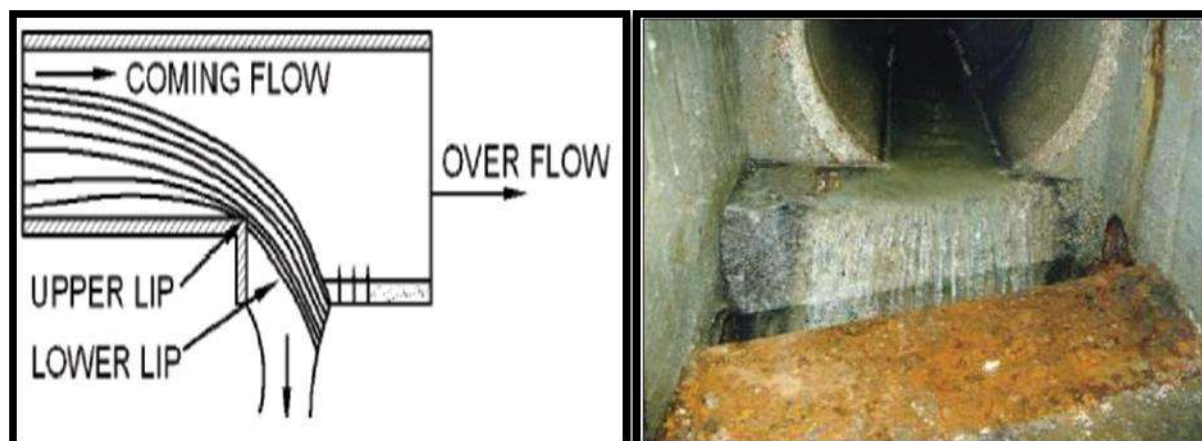
Figure 11.6: Leaping weir
