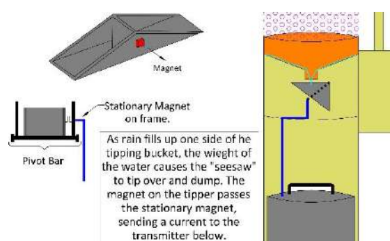
Figure 3. 1 Tipping bucket type rain gauge
