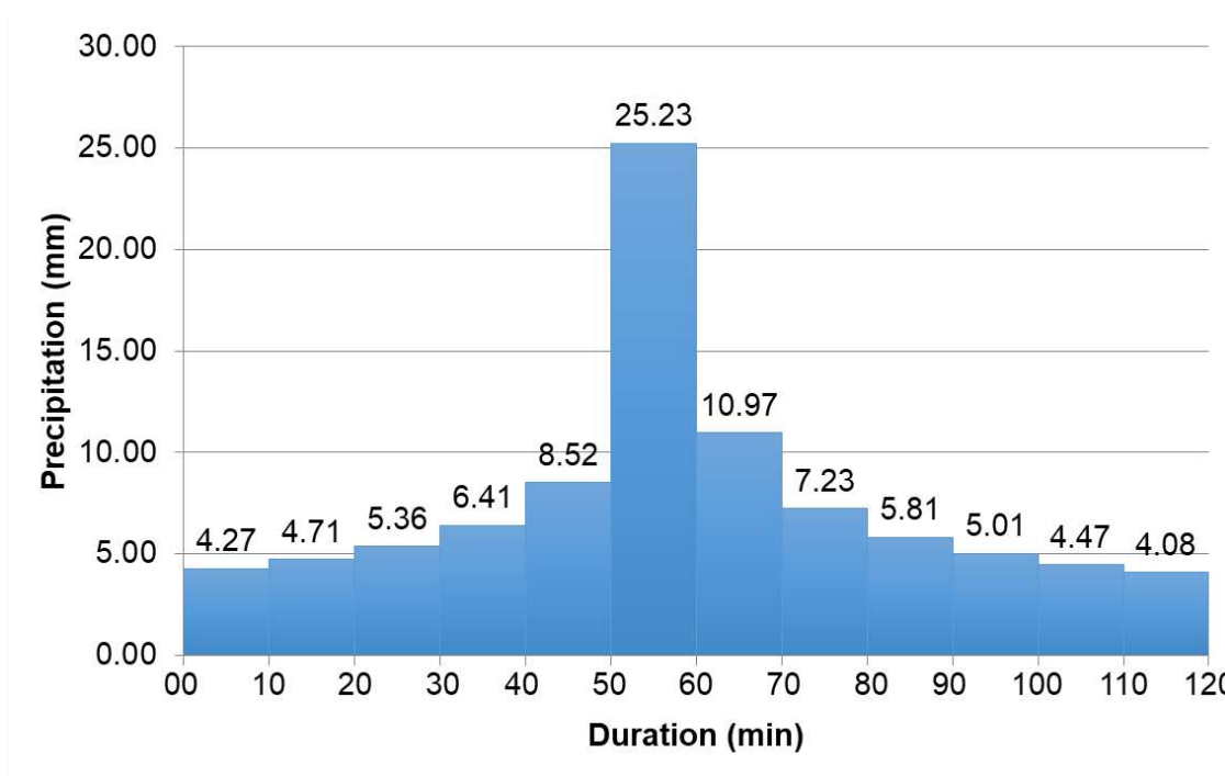
Figure 3.7: Hyetograph
