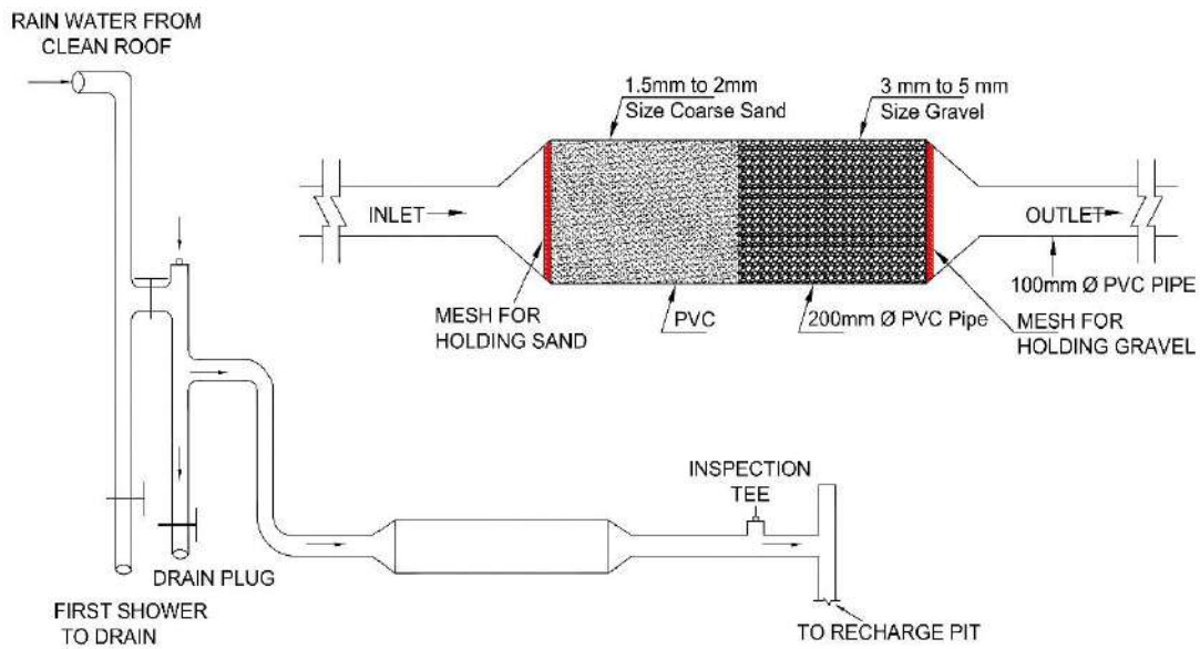
Figure 9.2: Filter unit
