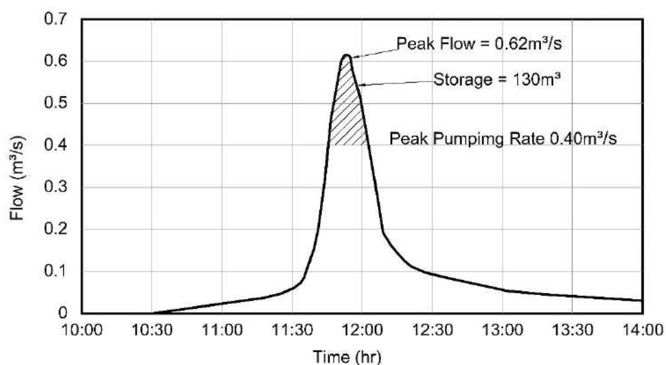
Figure 8. 3: Inflow Hydrograph
